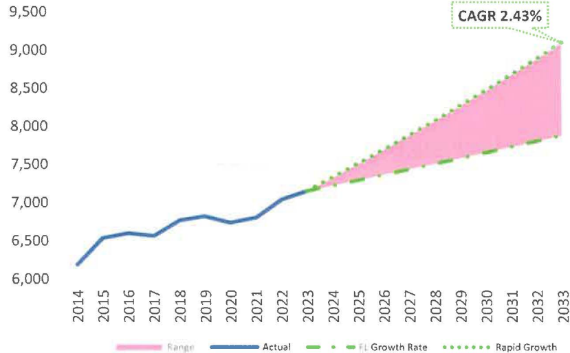
OUC Historic and Forecast of Energy Consumption, GWh 1
