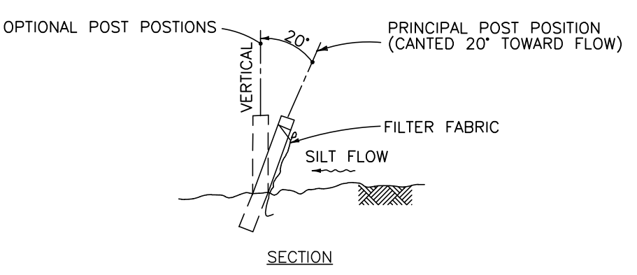
1 TYPE III SILT FENCE DETAIL NOT TO SCALE
