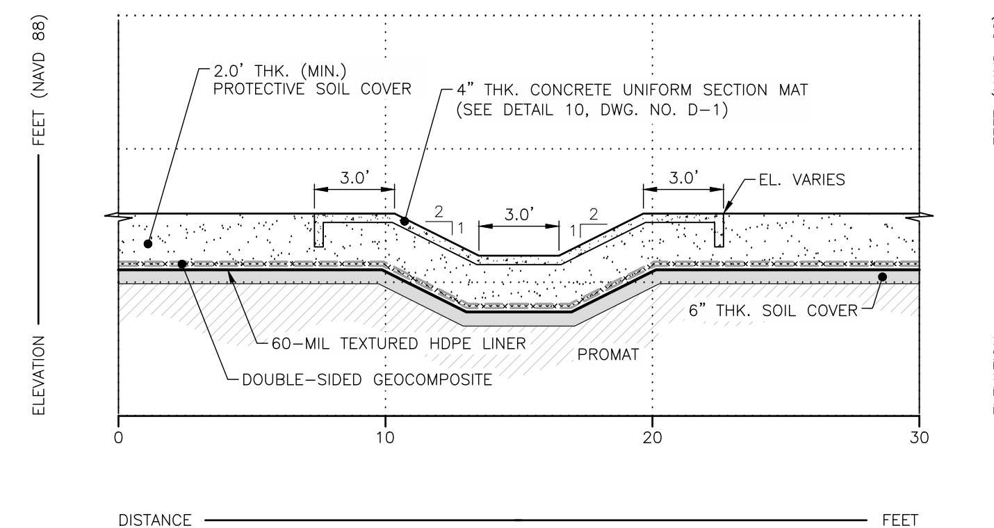
V FLUME ON SIDE SLOPE CS-5 CS-6 SCALE: 1" = 5'
