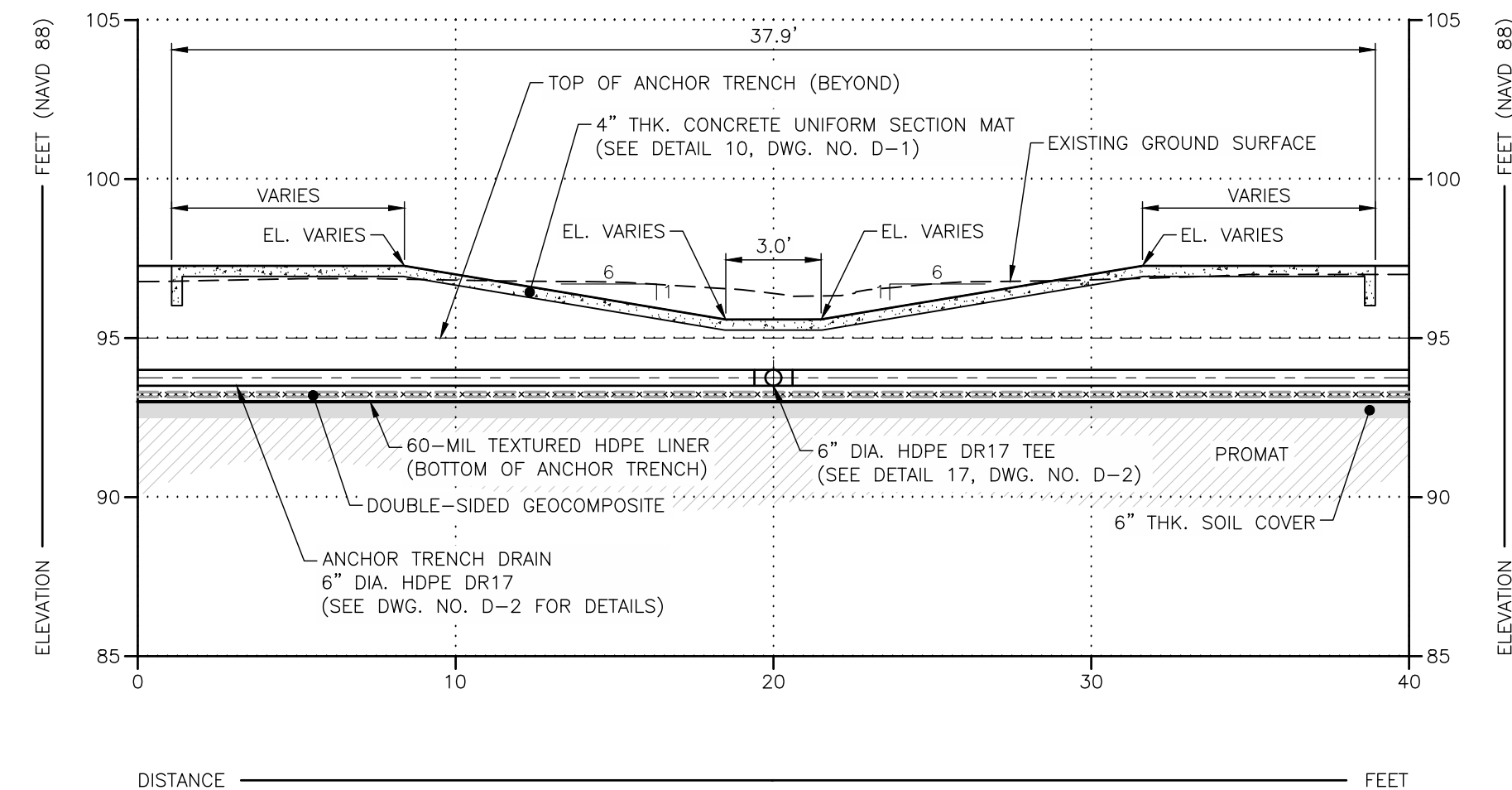
U FLUME CROSS SECTION AT CONTAINMENT DIKE CS-5 CS-6 SCALE: 1" = 5'
