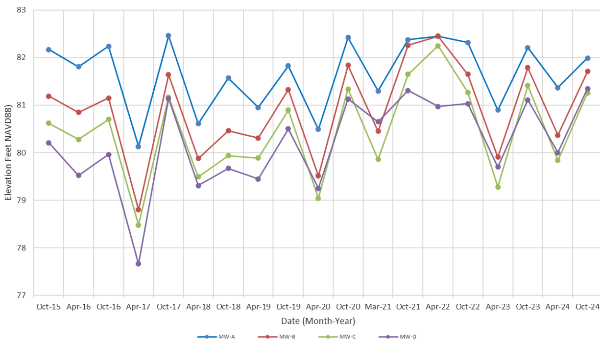
Figure 4: Semi-Annual Groundwater Levels
