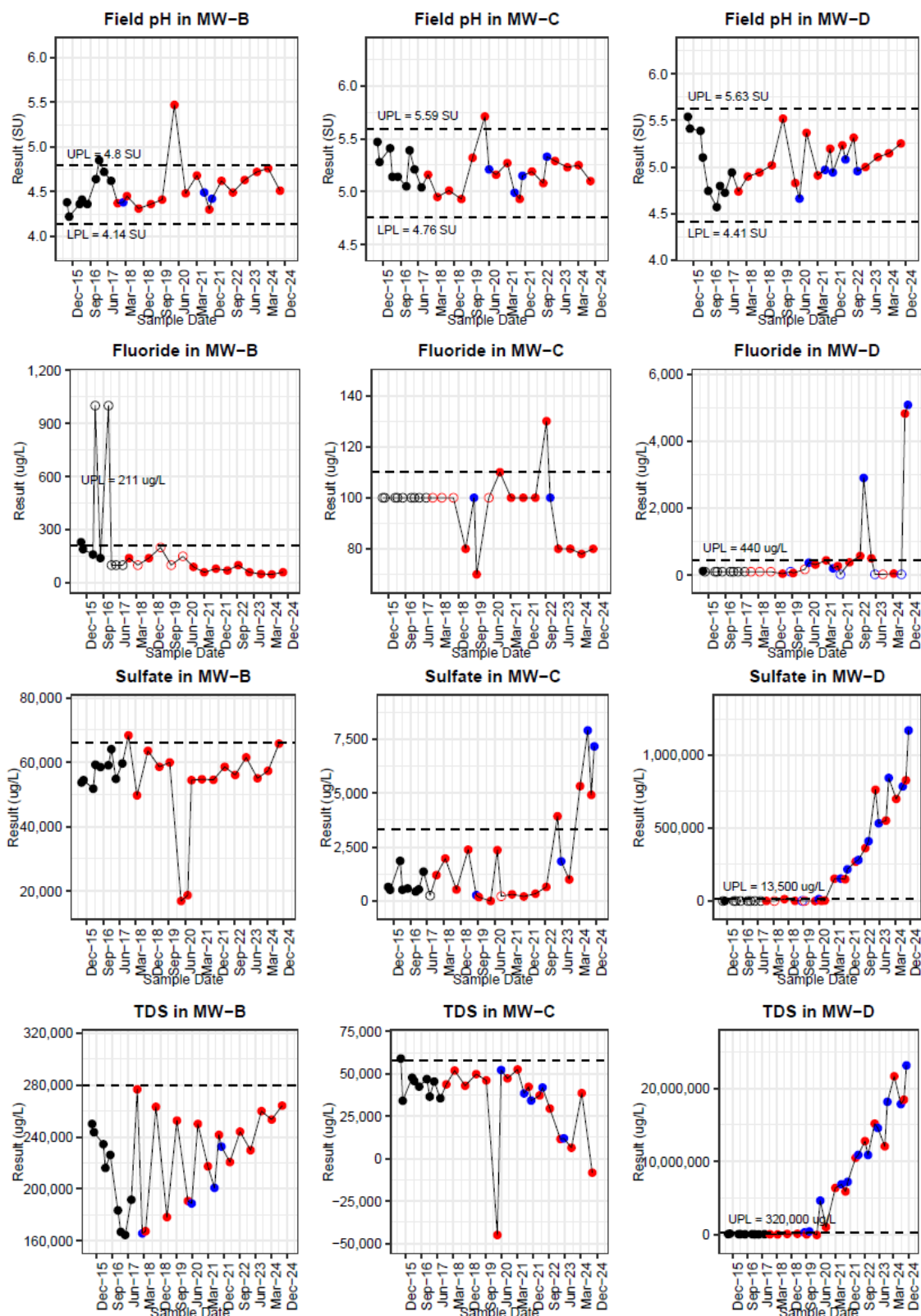
Figure 5: (Continued) Well-Constituent Results
